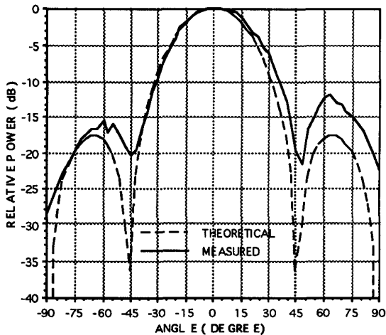
Figure 3a : Sum pattern in the azimuth plane.
