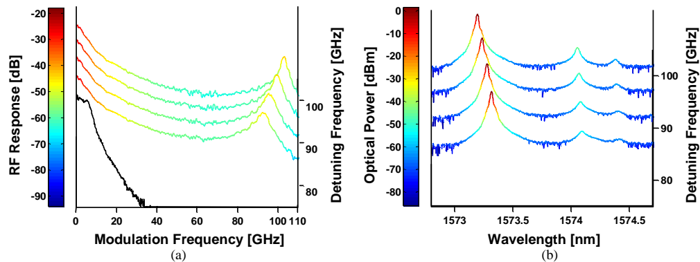
Fig. 5. Evolution of injection-locked VCSEL for different detuning frequencies: (a) frequency response (smoothed 0.5% for clarity) and (b) corresponding optical spectra for +13.6 dB injection ratio. The detuning frequencies are 88, 93, 98, and 102 GHz. The solid black line represents the free-running case. The curves are offset for clarity.
