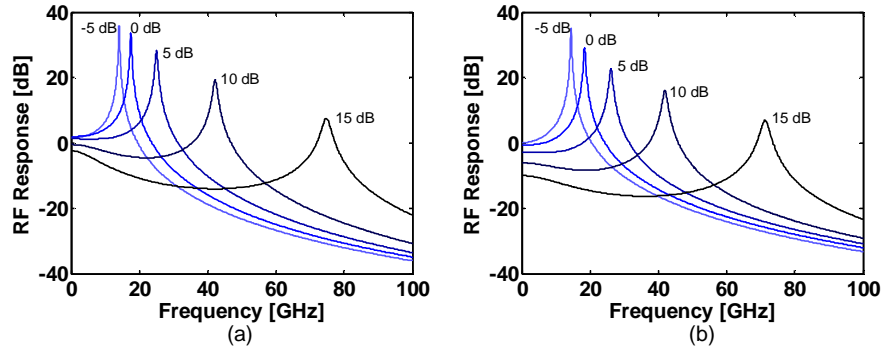
Fig. 1. Frequency response comparison between (a) DFB and (b) VCSEL, both with Q_c = 6800 . Each response curve shows the maximum resonance frequency for a given injection ratio, labeled on the curve. The maximum resonance frequency of each laser is the same for any given injection ratio.
